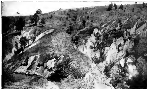
A. View illustrating struggle for existence among gullies.
